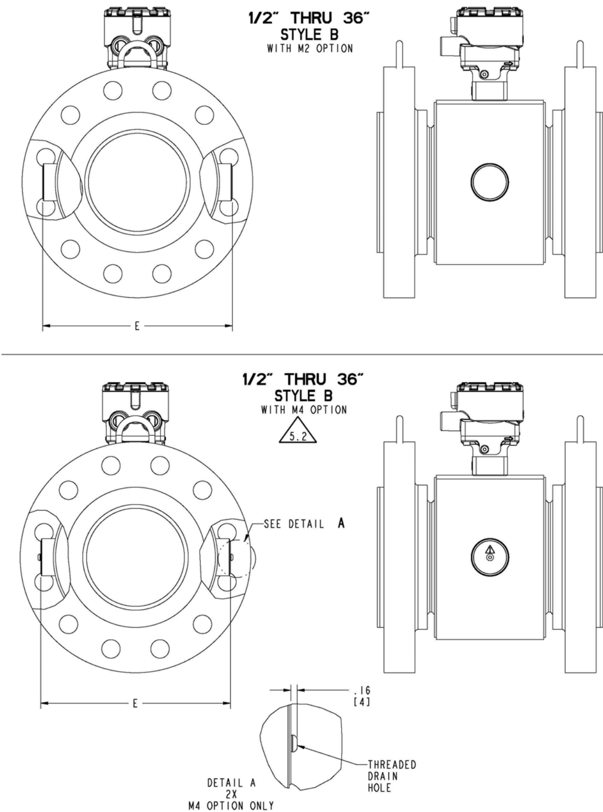
Figure 21: 8705-M Flanged Sensor 1/2 -in. to 36-in. (DN 15mm to 900mm) M2/M4 coil housing (P ≤ Class 2500)
