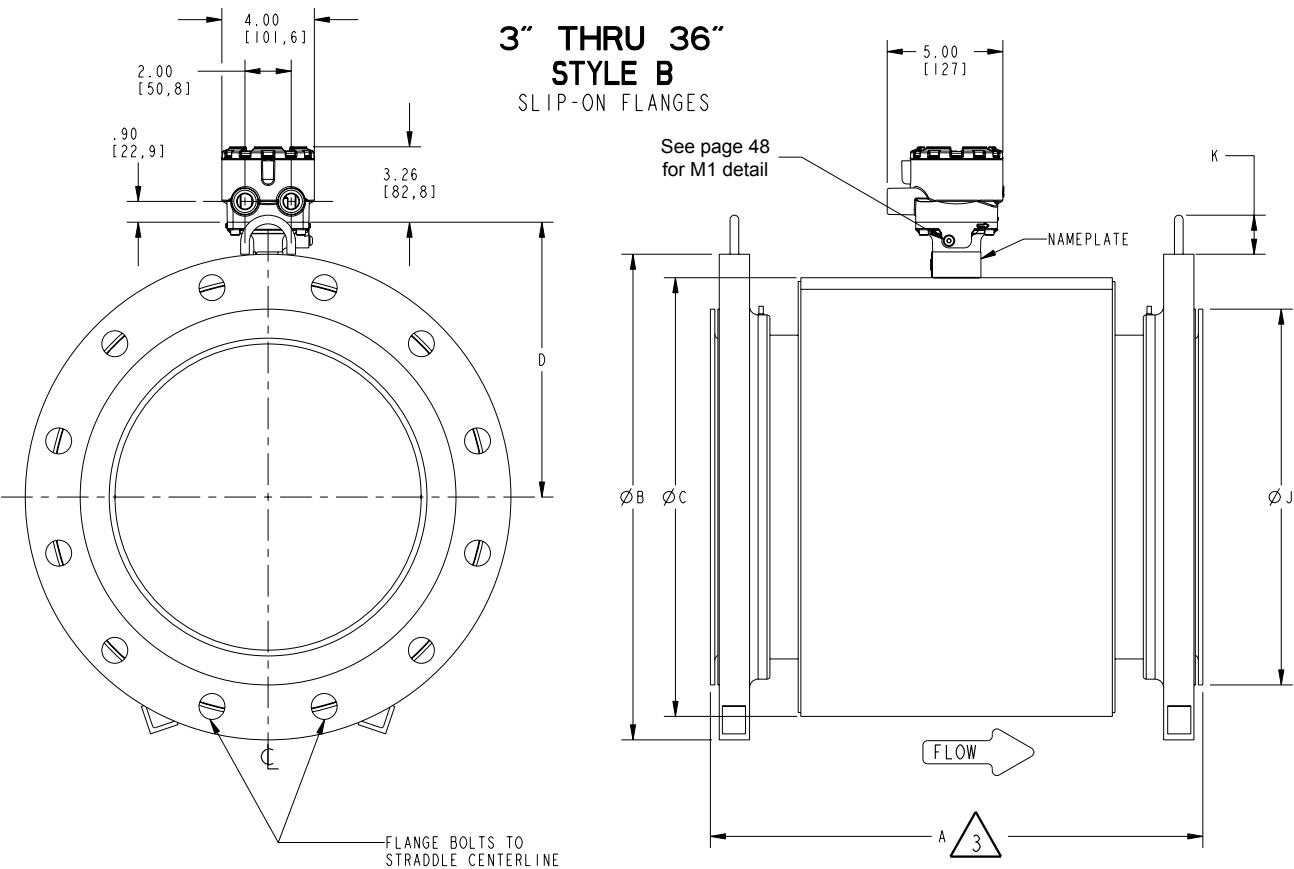
Figure 15: 8705-M Flanged Sensor 3-in. to 36-in. (DN 80mm to 900mm) slip-on flanges—low pressure ( P \leq \text{Class 300} )
