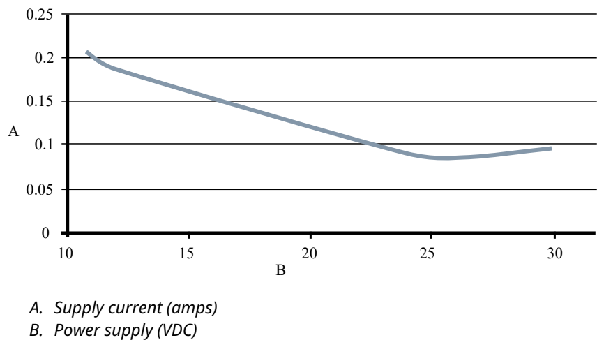
Figure 10: Low power DC current requirements
