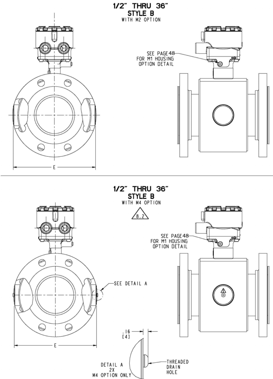
Figure 17: 8705-M Flanged sensor 1/2 -in. to 36-in. (DN 15mm to 900mm) M2/M4 coil housing (P ≤ Class 600 derated)
